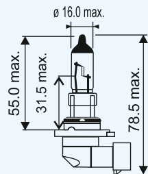
HB4/9006
