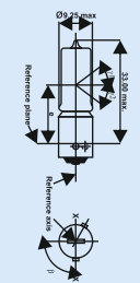
H21W
