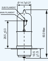
M5-TP
