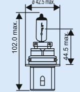
HB5/9007
