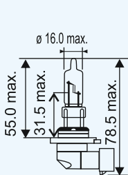
HB3/9005
